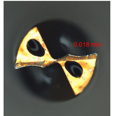
Tool wear < 20 µm after 3421 holes
